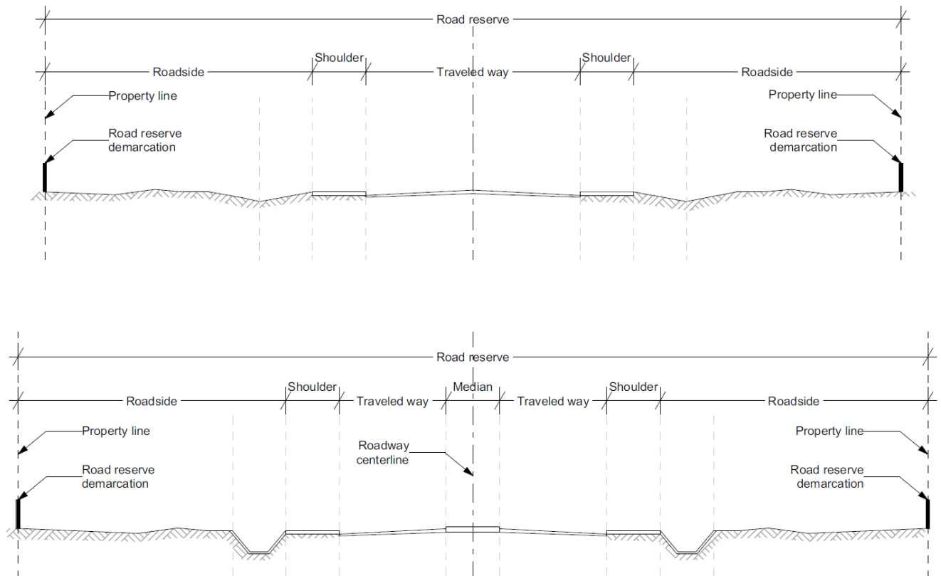
Figure 1b — Typical section illustrating the road reserve
