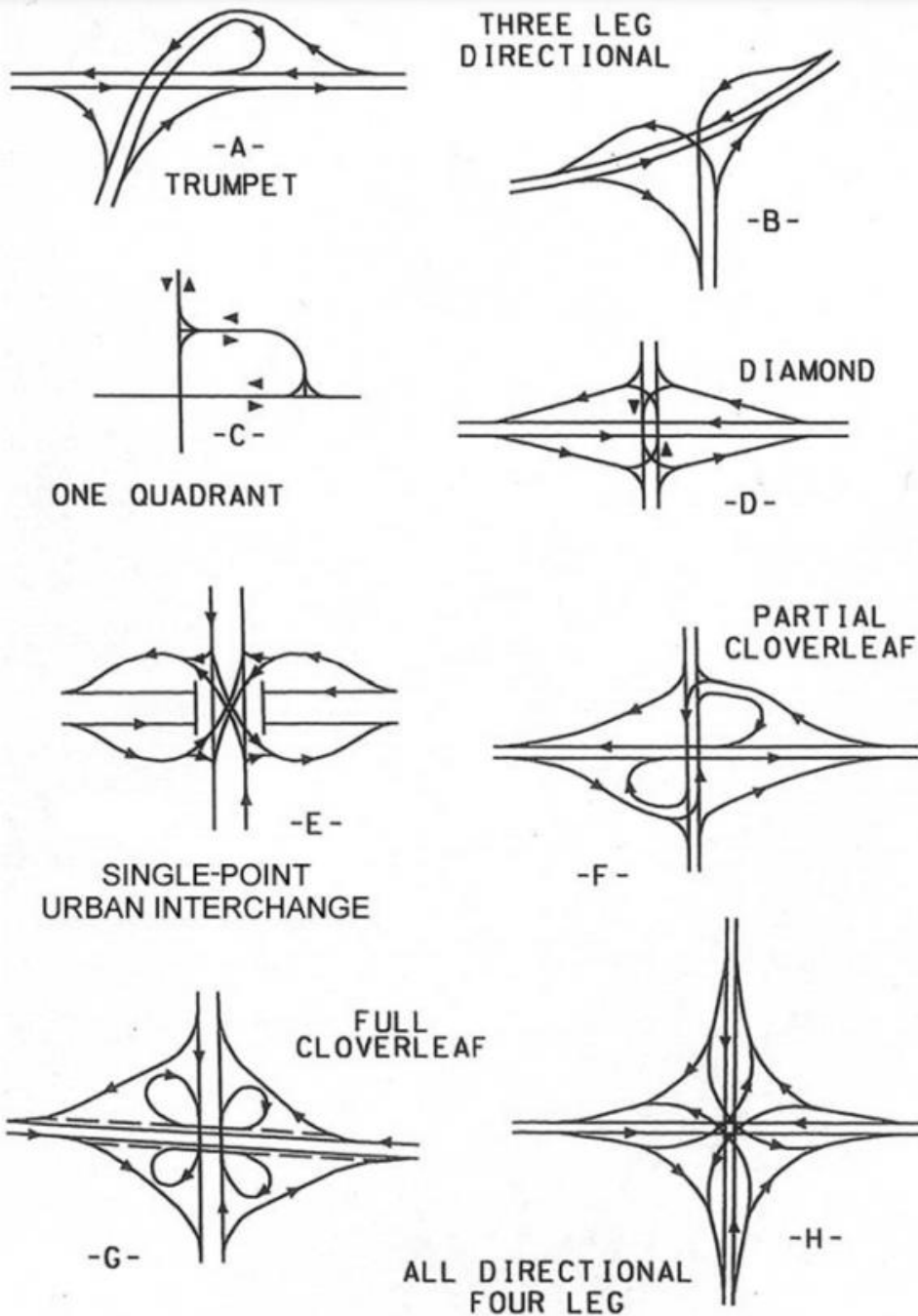
Figure 20 — Interchange Configurations
