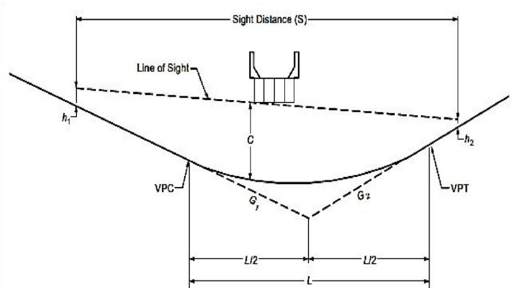
Figure 15 — Schematic view of sight distance at undercrossing
