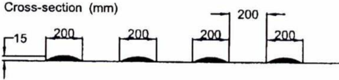
Figure 22 — Design of rumble strips option two
