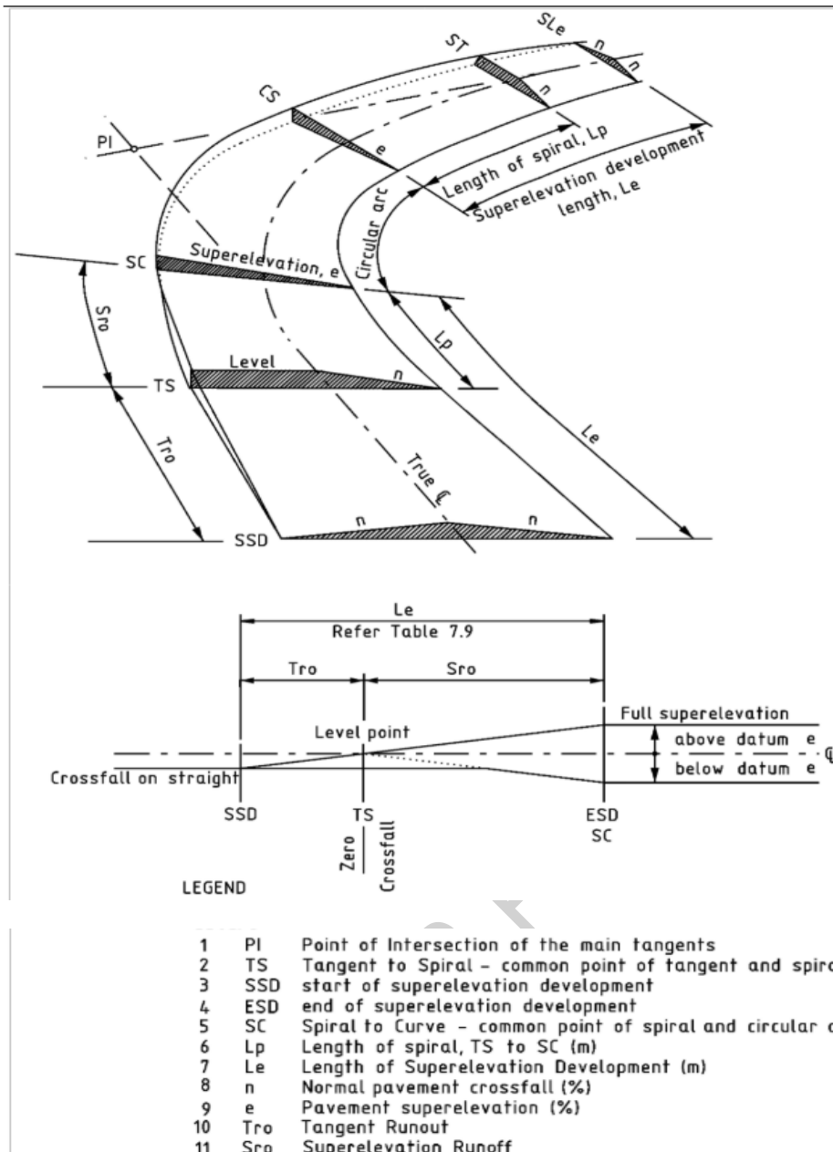
Figure 2 — Elements of Super-elevation and transition curve
