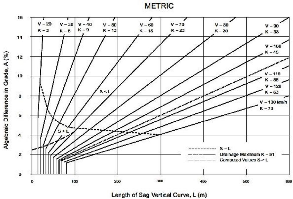
Figure 14 — Length of sag vertical curve as a function of algebraic difference in grade A (%)
