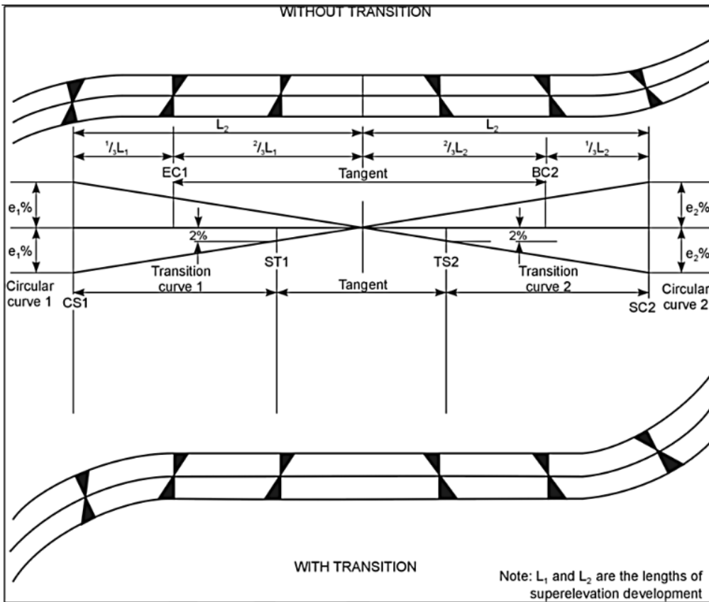
Figure 3 — Super-elevation of Reverse Curves
