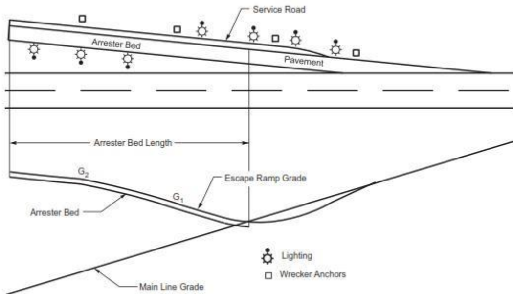
Figure 18 —Typical emergency escape ramp
