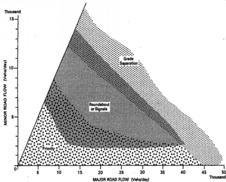
Figure 19 —Types of intersections appropriate to different traffic flows
