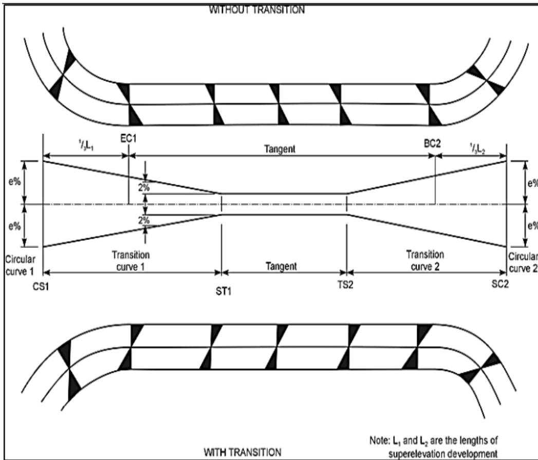
Figure 4 — Super-elevation of broken-back curve
