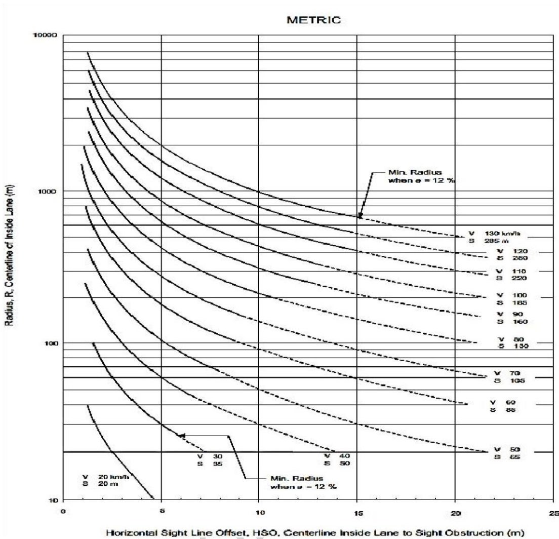
Figure 6 — Diagram illustrating components for determining horizontal sight distance
