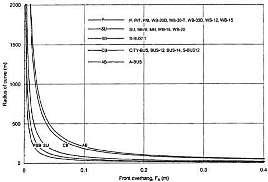
Figure 10 Front Overhang for Widening of Traveled Way on Curves
