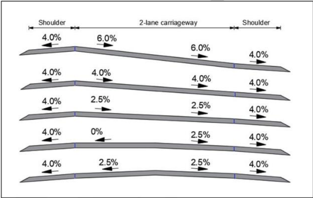
Figure 8 — Super-elevation of a two-lane carriageway about the centerline
