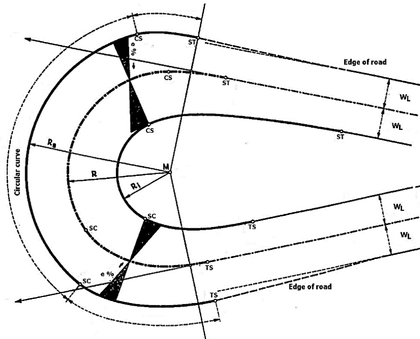
Figure 12. Switchback Curve Layout
