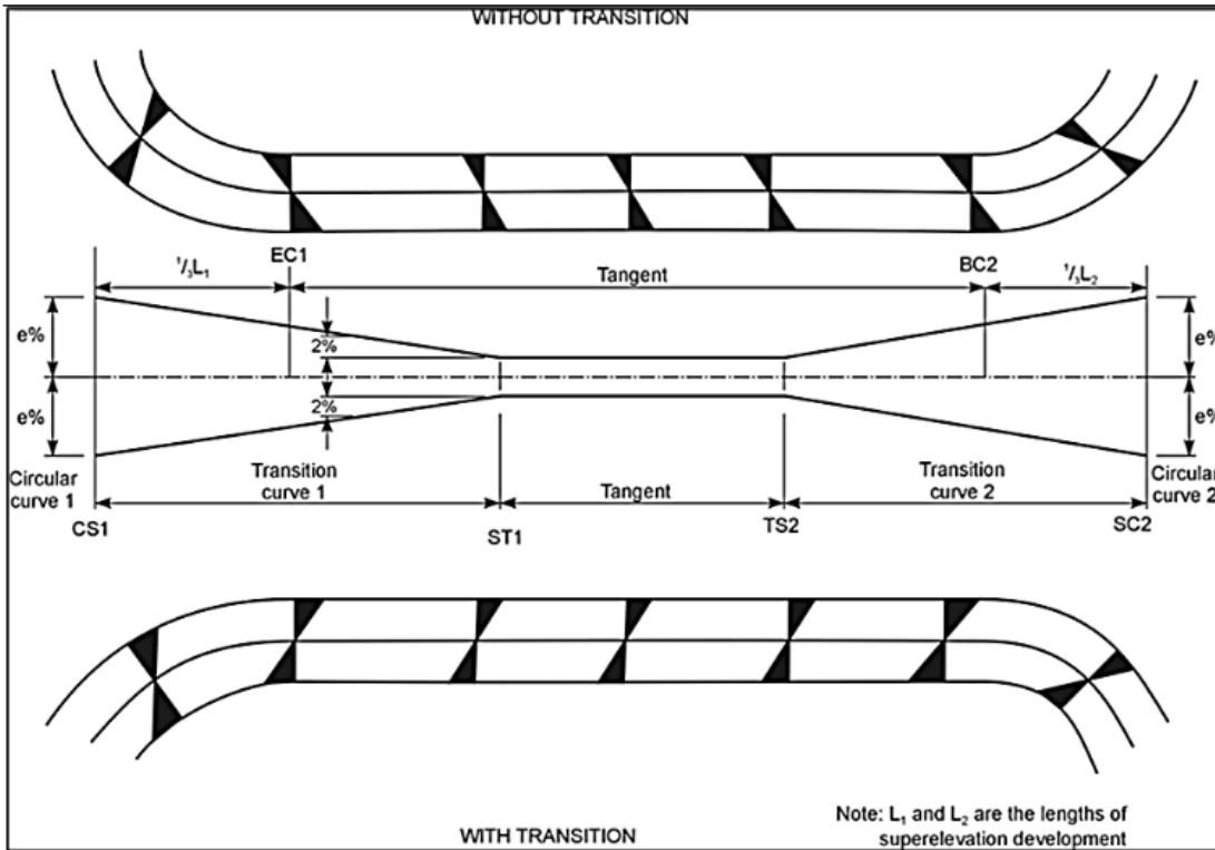
Figure 5 — Super-elevation of compound curve
