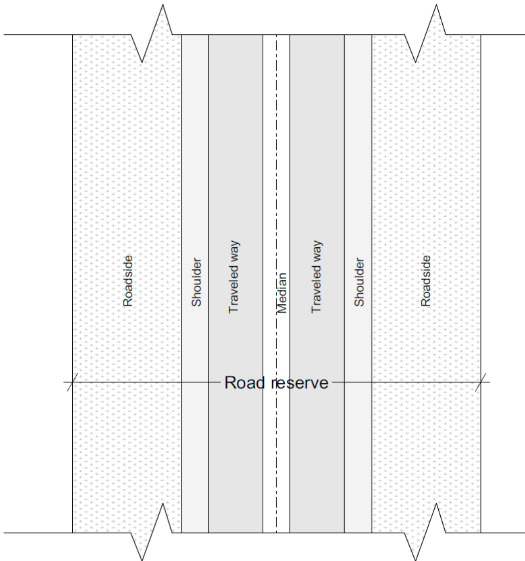
Figure 1a — Plan view of roadway illustrating road reserve
