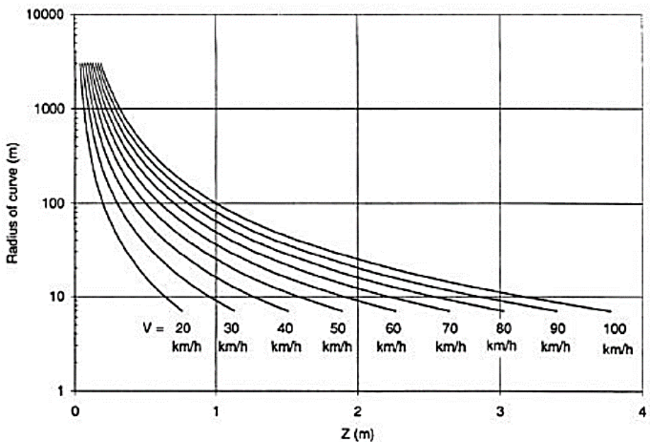
Figure 11 —Extra Width Allowance for Difficulty of Driving on Traveled Way
