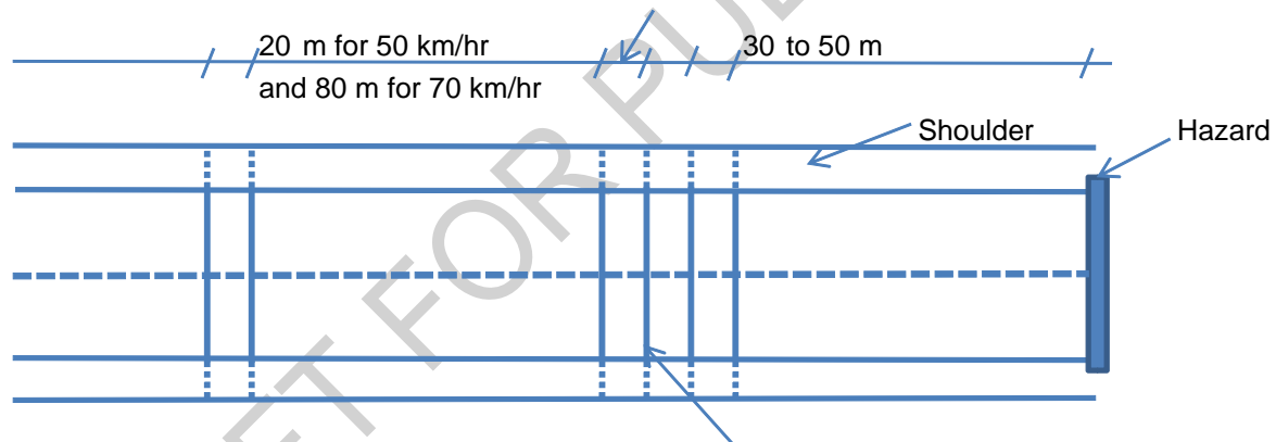
Figure 21 — Design of rumble strips option one
